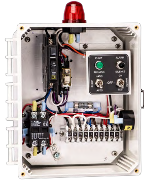
Simplex Control PN: 50A006
