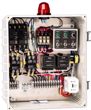
Duplex Control PN: 50A506
