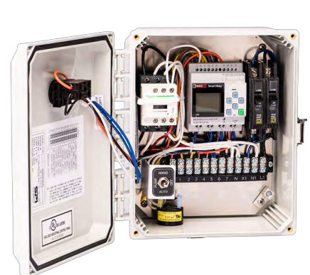
Time-Dosed Panel PN: 50A808
