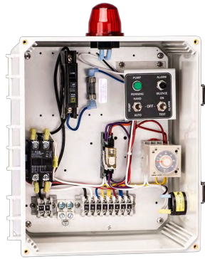
Time-Dosed Panel PN: 50A801
