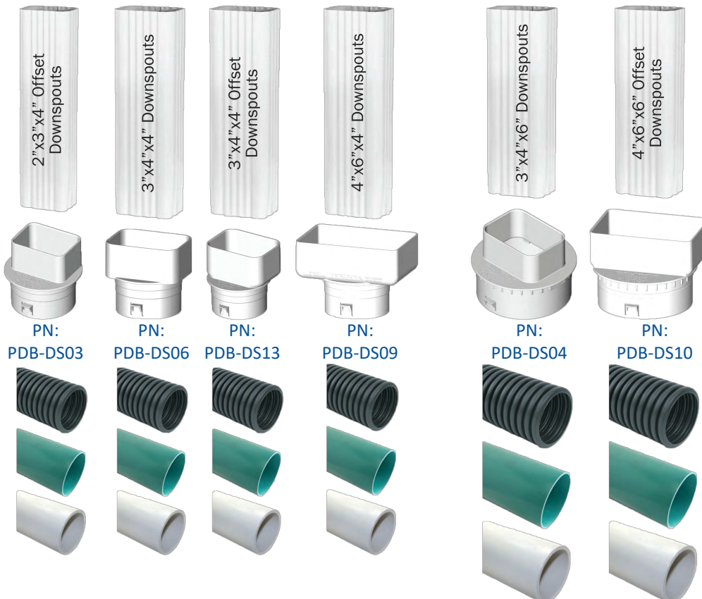
4" AND 6" CORRUGATED PIPE ADAPTERS
